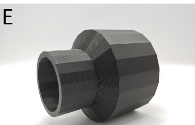
A-C: CAD model of proposed 3D printed mask body D: Endcap for PVC mask E: 4" suction hose to 2" spigot adapter
